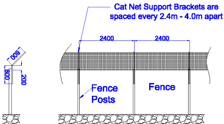
Typical fence mounted Cat Net installation details
